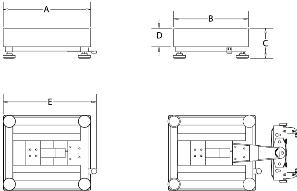
Figure 1. Defender Base Dimension Drawing.
